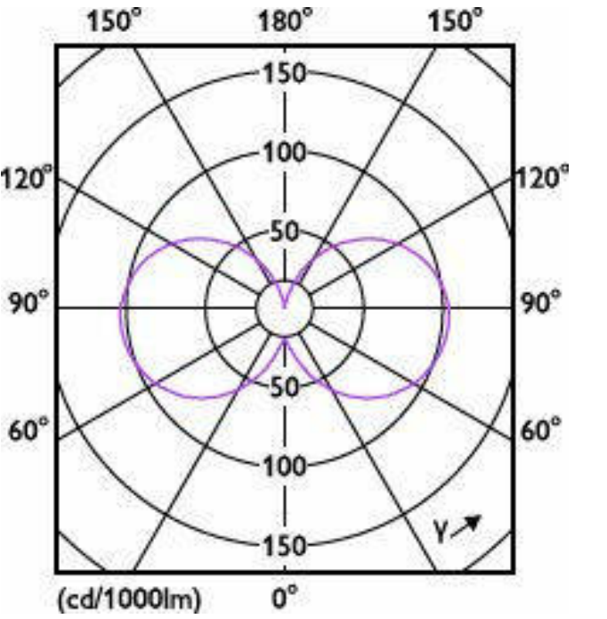
Light Distribution Diagram - CorePro LED PLC 360D 9.5W 3CCT 4P G24q-3
