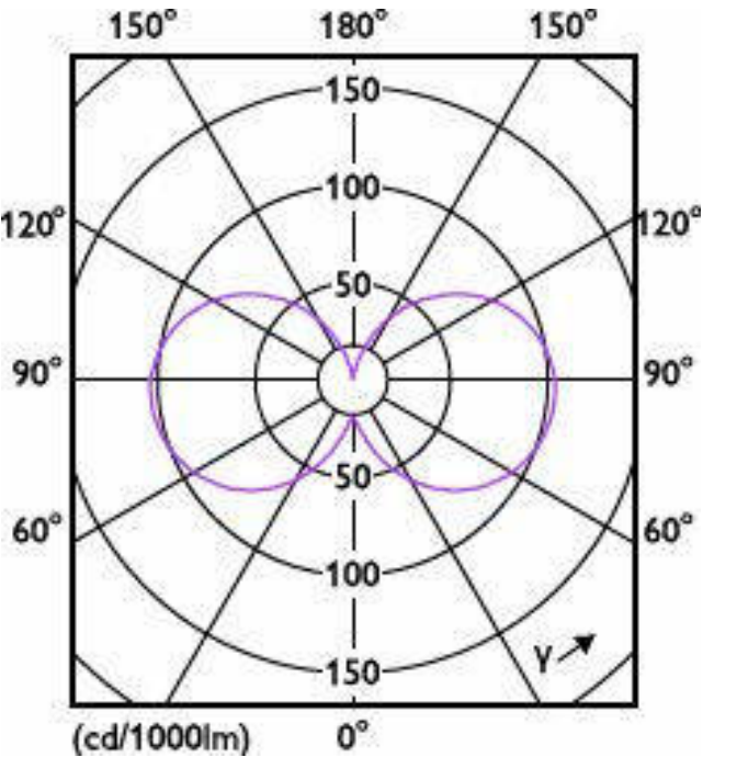
Light Distribution Diagram - CorePro LED PLC 360D 5.5W 3CCT 4P G24q-1
