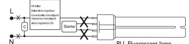
PLL Fluorescent lamp
