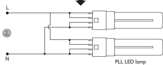
PLL LED lamp
