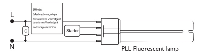
PLL Fluorescent lamp
