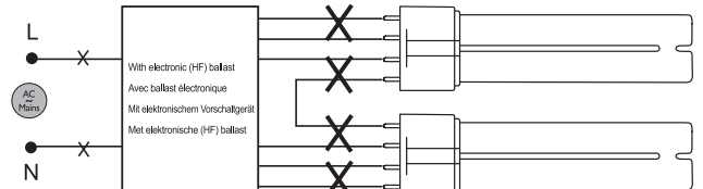
PLL Fluorescent lamp
