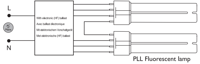
PLL Fluorescent lamp
