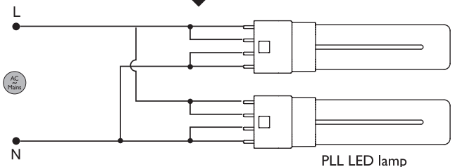
PLL LED lamp
