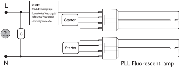
PLL Fluorescent lamp
