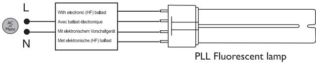
PLL Fluorescent lamp
