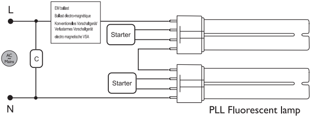
PLL Fluorescent lamp
