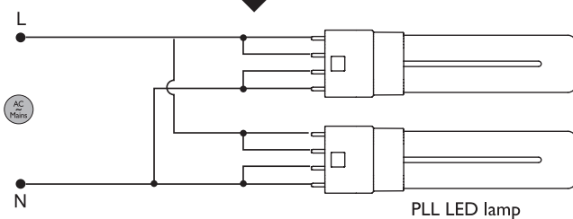
PLL LED lamp
