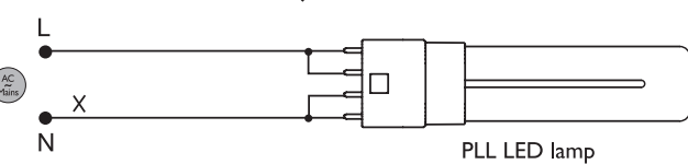
PLL LED lamp
