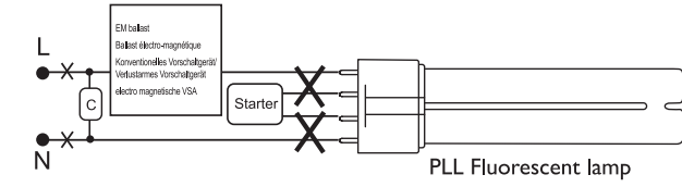
PLL Fluorescent lamp
