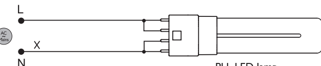
PLL LED lamp
