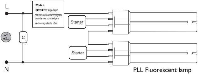
PLL Fluorescent lamp
