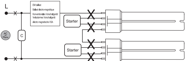
PLL Fluorescent lamp
