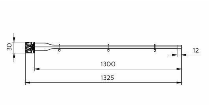
WT120Z TW-3x2.5-L1500
