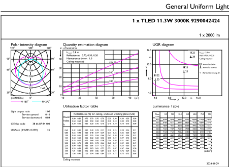
Light Distribution Diagram - MAS LEDtube 1200mm HO 11.3W 830 T8 EELC
