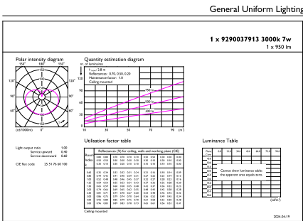
Light Distribution Diagram - CorePro LEDlinear ND 7-60W R7S 78mm830
