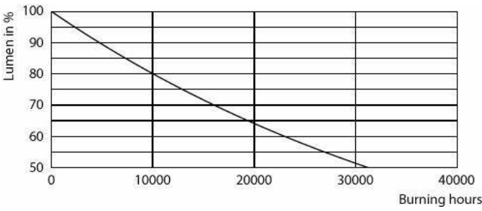
Lumen Maintenance Diagram - CorePro LEDcapsuleLV 1-10W G4 827micro
