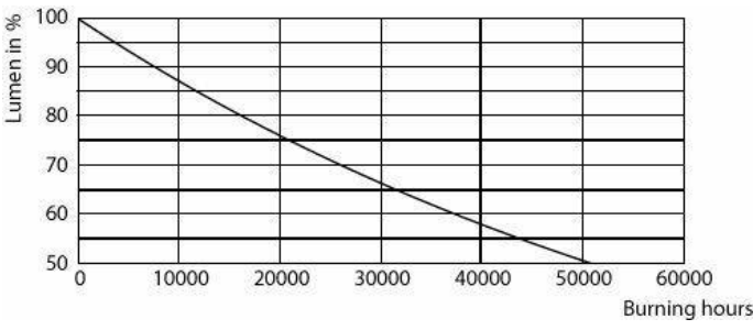
Lumen Maintenance Diagram - TForce Core LED road 49W 740 E40 MV
