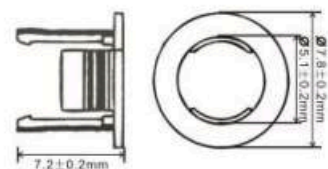
Indicator holder
