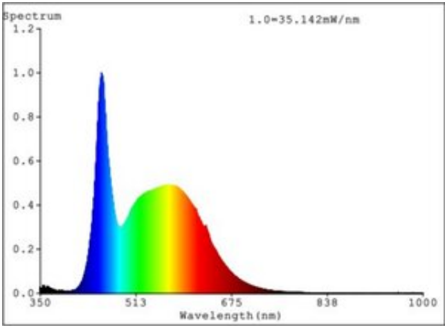
VALUE CLA75 10W 865
