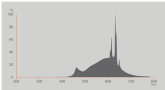
EPREL Data Spectral Diagram LEDr_CRI90_Blue light reduced_2700K
